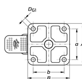
Rectangular Top Plate Fixing
