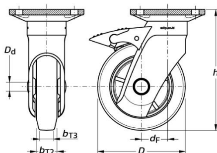
SIJB-100-P & SIJB-127-P Swivel Castors with Total Brake
